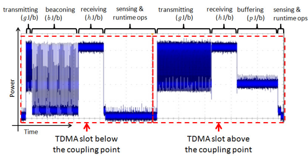
Figure 2. Energy profile of a TelosB sensor node within an undercoupled and an overcoupled TDMA slot during the active period. The indicated metrics (in Joule-per-bit) are defined in Table I.
