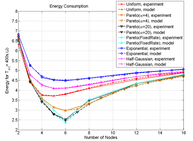
Figure 5. Energy consumption per node under different data transmission PDFs. The experiments correspond to T_{act} = 400 s, k = 165.6 mJ and d = 0 .
