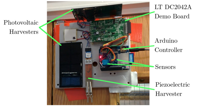
Figure 1. Energy harvesting platform with annotations on key components.
