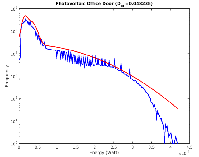
Figure 2. Histogram of photovoltaic harvester (blue) on ‘‘Office door’’ and best fit (red) obtained via (4).
