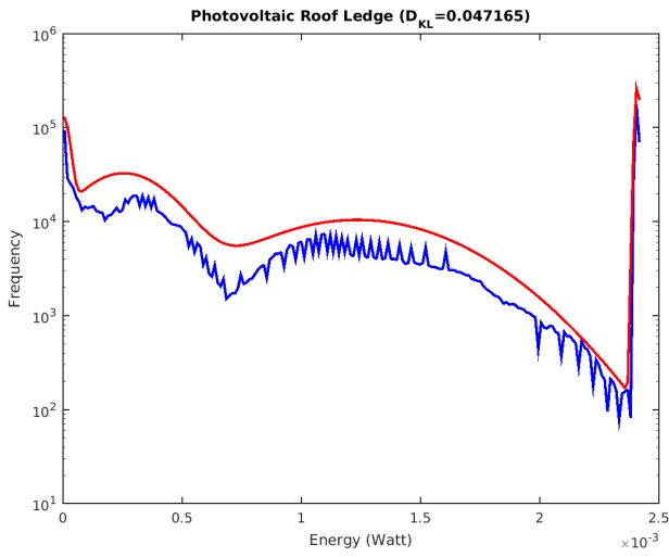
Figure 4. Histogram of photovoltaic harvester (blue) on ‘‘Roof ledge’’ and best fit (red) obtained via (6).
