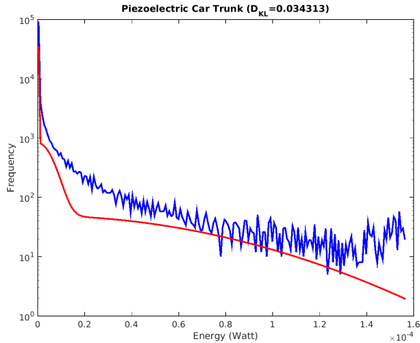
Figure 7. Histogram of piezoelectric harvester (blue) on “Car trunk” and best fit (red) obtained via (9).
