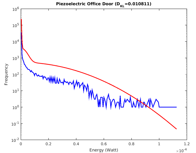
Figure 3. Histogram of piezoelectric harvester (blue) on ‘‘Office door’’ and best fit (red) obtained via (5).
