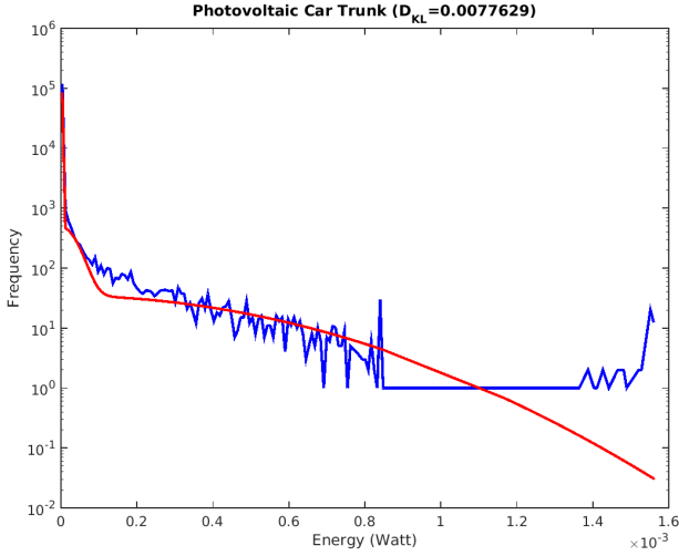
Figure 6. Histogram of photovoltaic harvester (blue) on “Car trunk” and best fit (red) obtained via (8).
