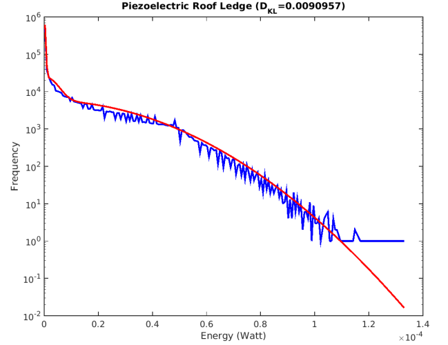
Figure 5. Histogram of piezoelectric harvester (blue) on ‘‘Roof ledge’’ and best fit (red) obtained via (7).
